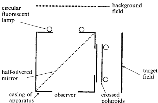
Figure 1. Plan of the apparatus used to superimpose the target letter on the background grating (experiments 1 and 2).
